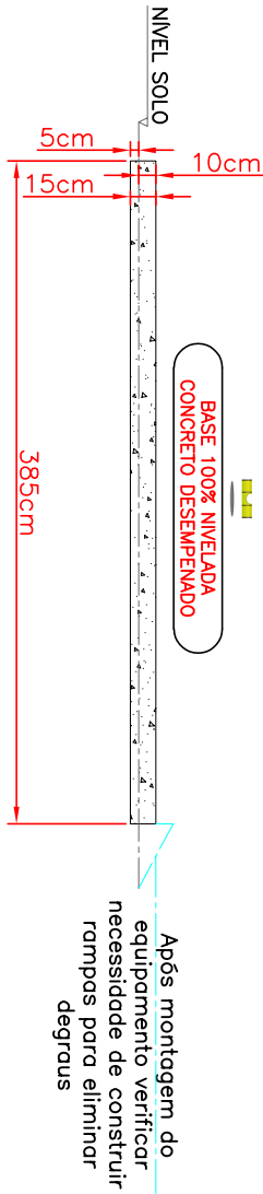
– Vista Lateral Base
