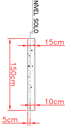
– Vista Frontal Base
